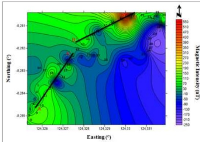
Figure 5. Slices in the regional anomaly contour map
