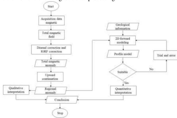
Figure 2. Flowchart for processing magnetic data
