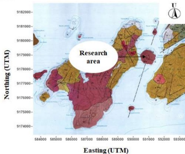
Figure 1. Geological map of Pantar-Pura
